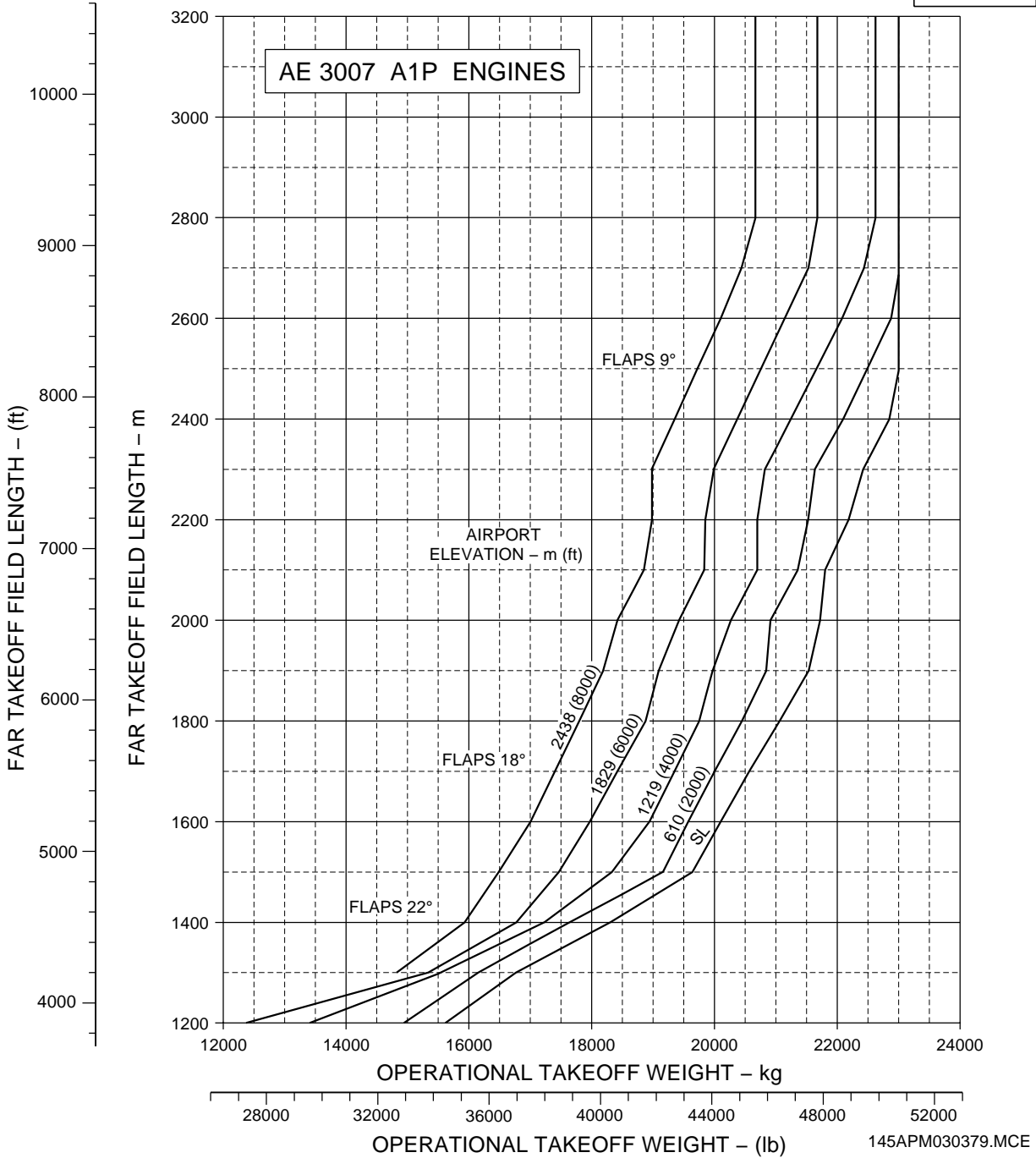
Figure 3.3.2 - FAR Takeoff Runway Length Requirements - ISA + 15°C Conditions Sheet 4
