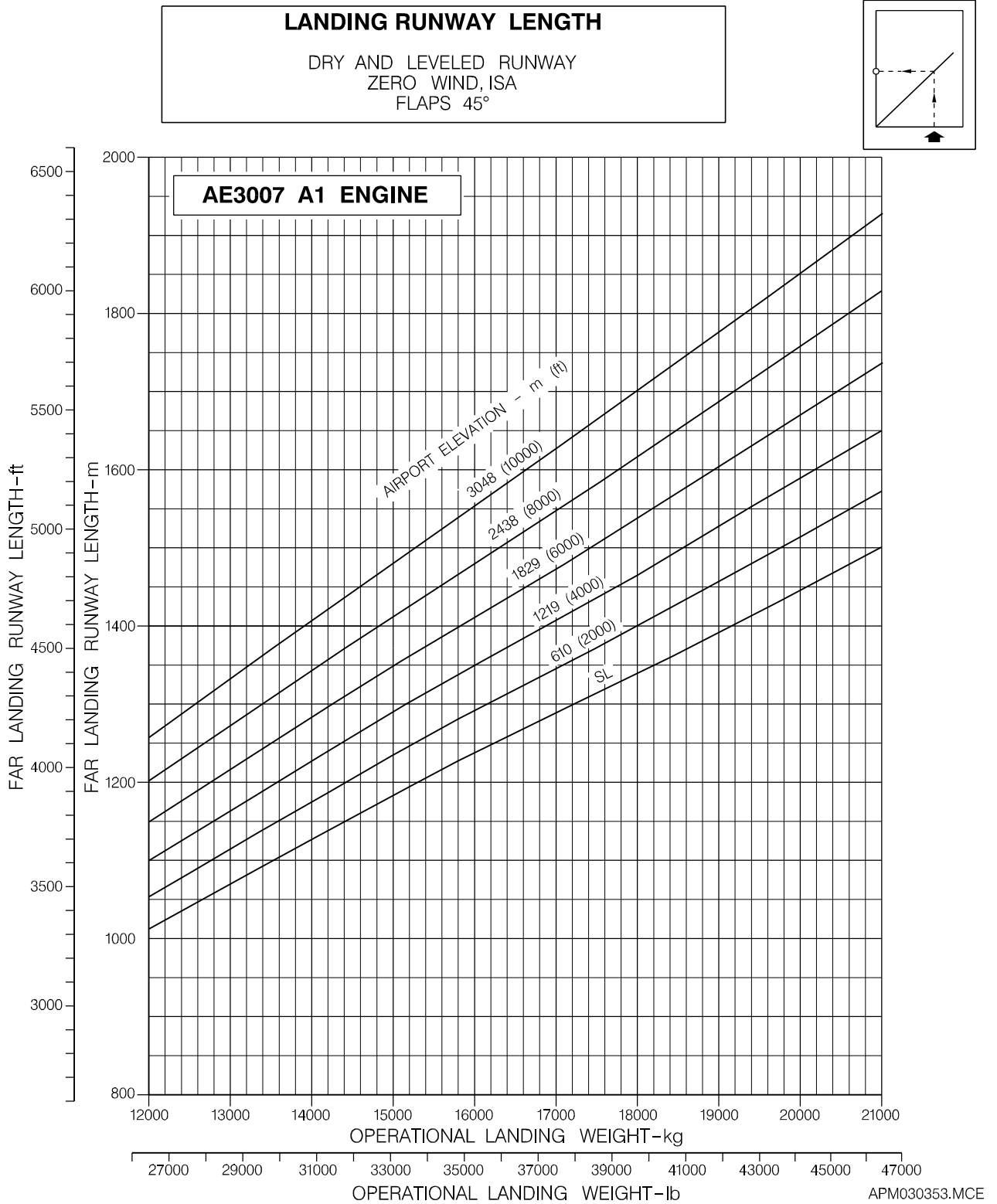
Figure 3.4.1 - FAR Landing Runway Length Requirements - Flaps 45° Sheet 1
