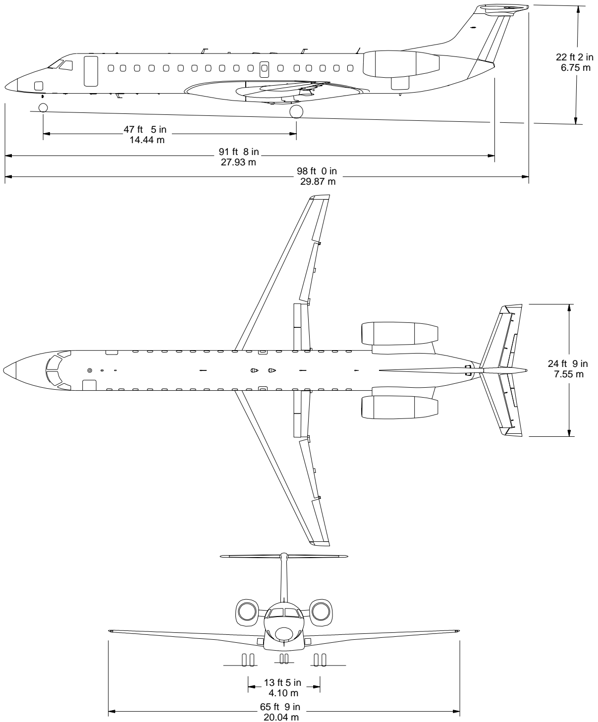
EMB-145 EP/ER/EU/MP/MK/LR/LU
