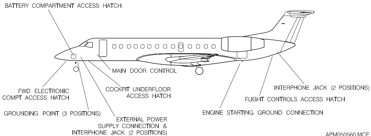
Figure 5.4.1 - Ground Servicing Connections EMB-145 ER / MP
